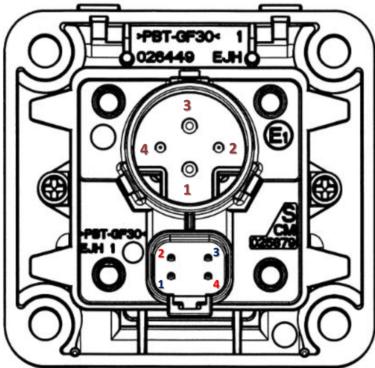
Connection - tractor side
